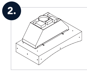
2. Assemble blower unit (sold separately) to metal liner
