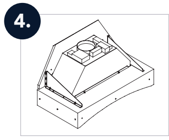
4. Hang the liner/bracket assembly on the mounting plate (make all electrical and ventilation connections at this point)
