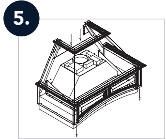
5. Slip the wood range hood on top of the mounting plate
